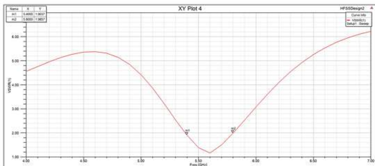
Figure 5: Simulated VSWR vs. Frequency plot of the proposed FPDA.
