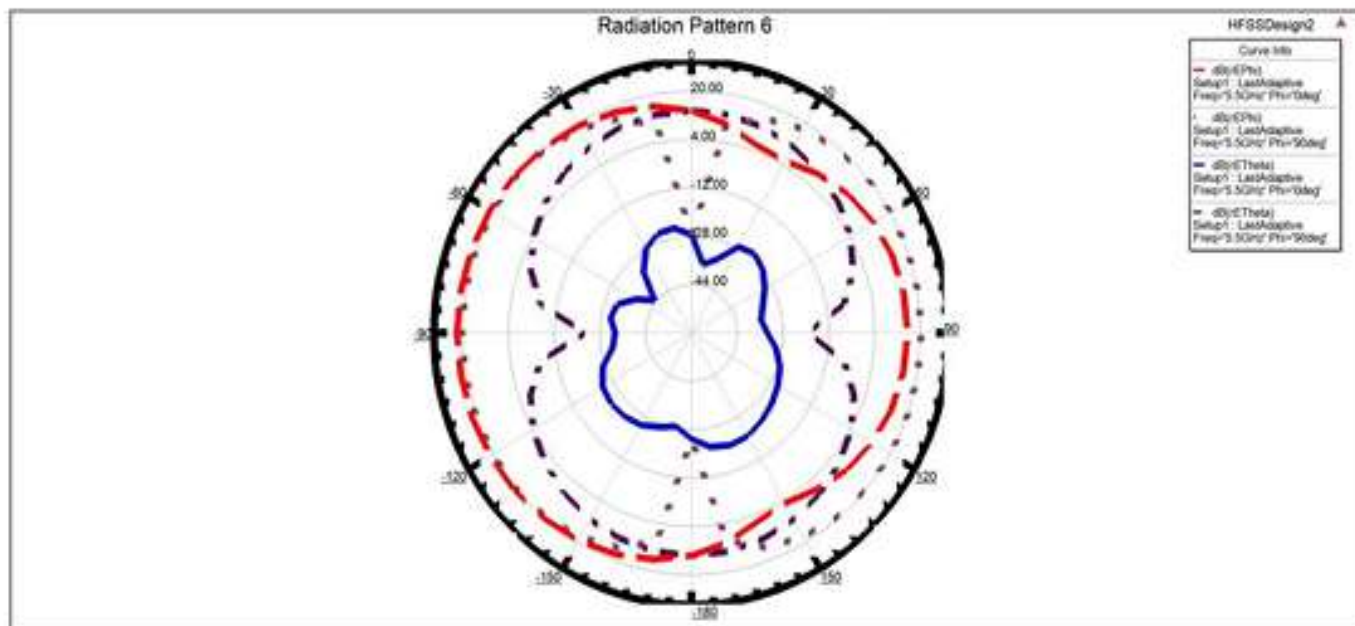
Figure 4: Radiation Pattern at 5.5 GHz
