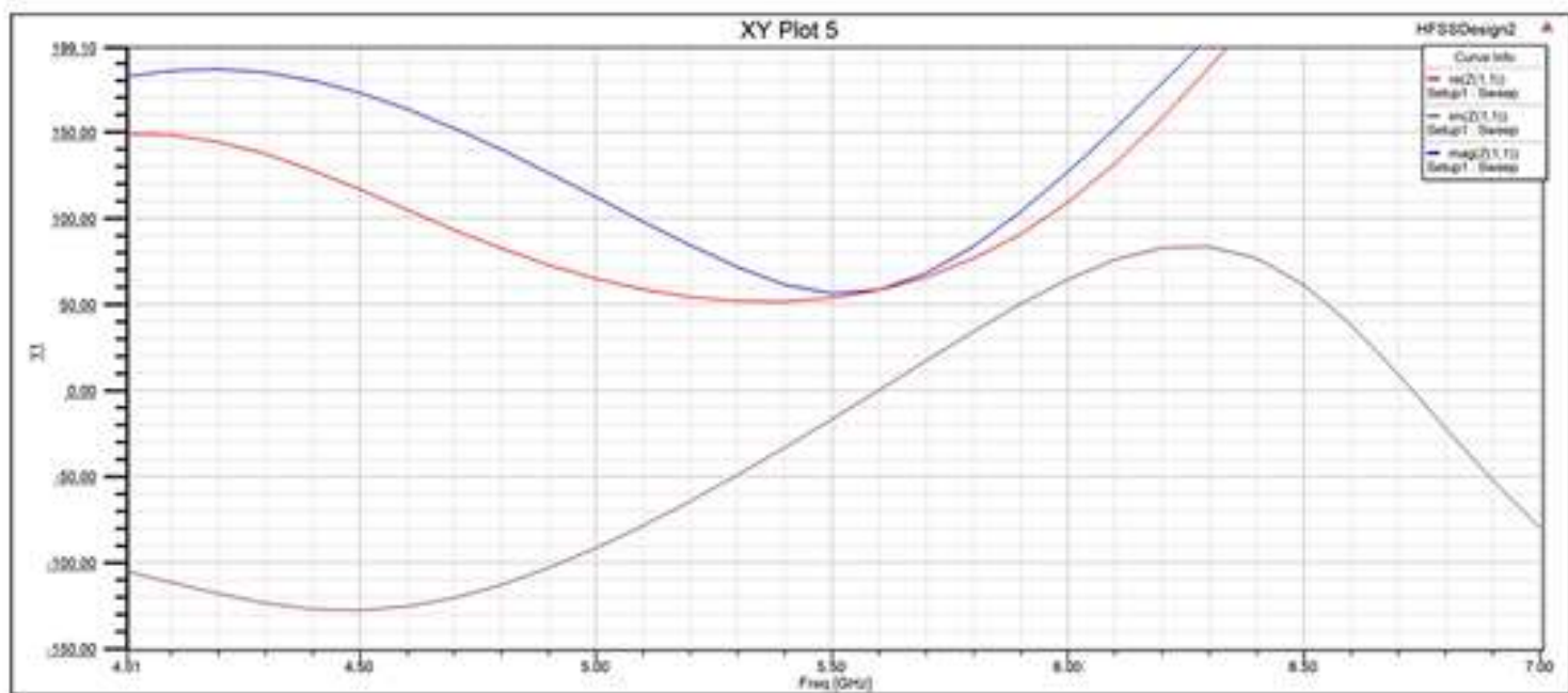
Figure 4: Graph of frequency vs impedance variation.
